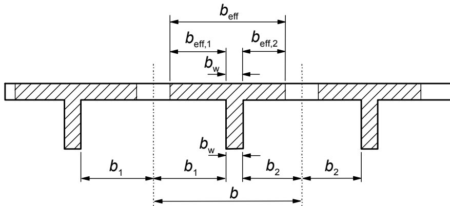
Figure 5.3: Effective flange width parameters
