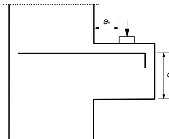
(b) Corbel
