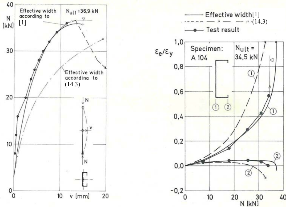
Figure 14.2: Results from tests on studs with thin-walled C-section under compression together with calculated values with two different estimates of the effective width [1]
