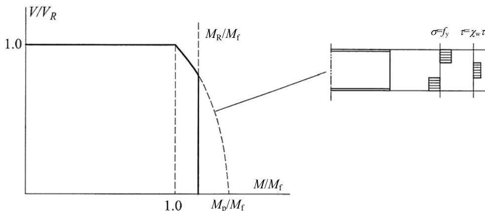
Figure 7.3: Interaction between bending moment and shear according to Basler
