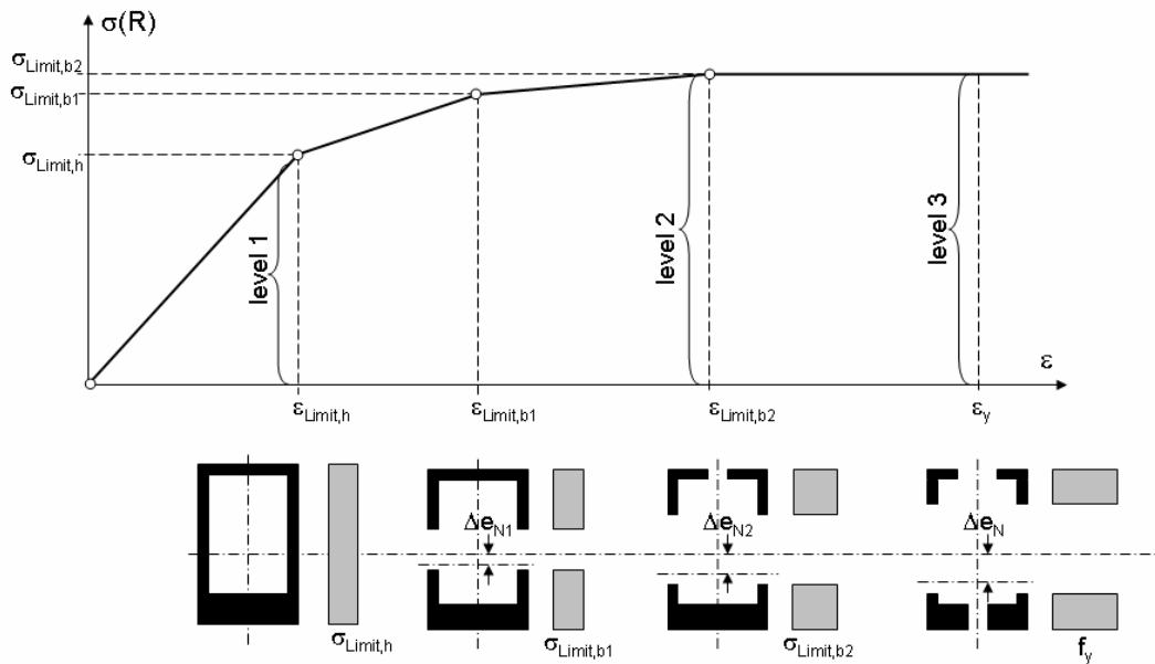
Figure 2.9: Development of eccentricity of neutral elastic axis versus the strain \varepsilon
