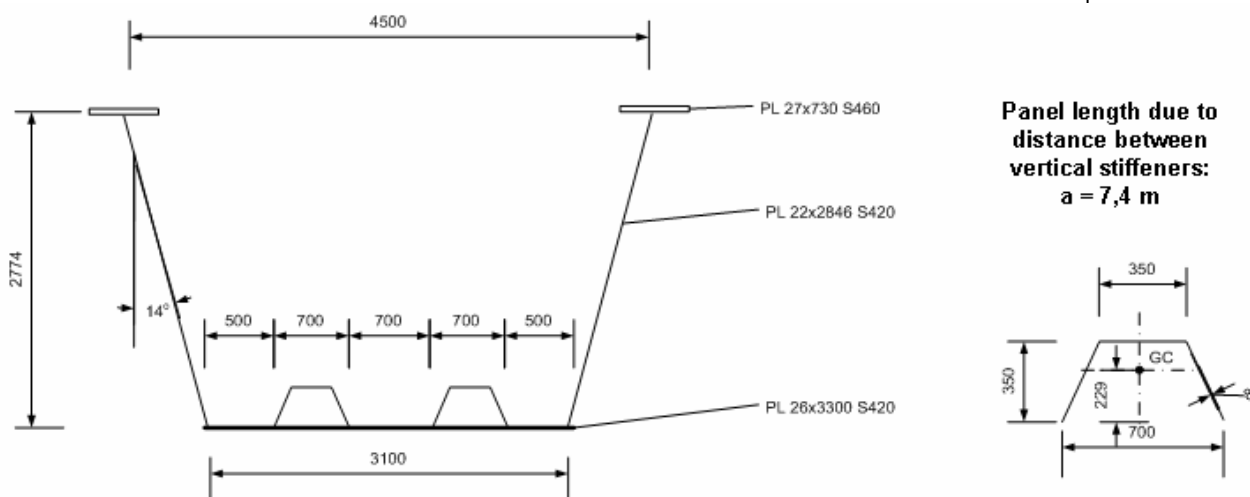
Figure 15.2: Cross section at pier 2 when the nose reaches pier 3
