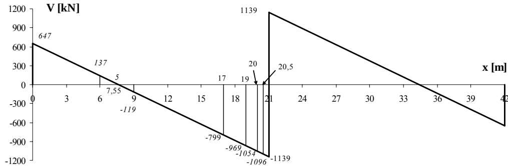
Figure 17.3: Shear force
