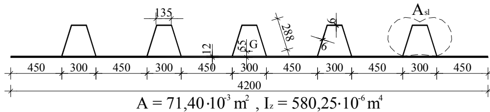
Figure 16.3: Gross cross section
