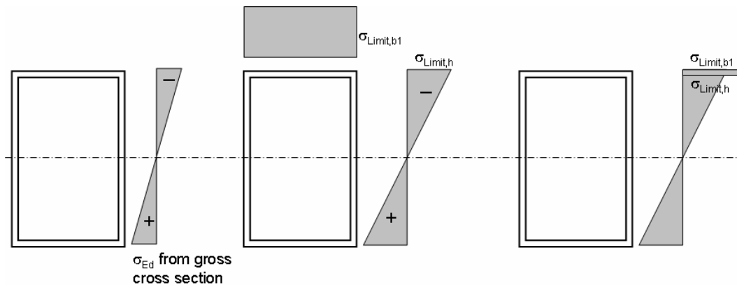
Figure 2.10: Distribution of plate buckling strength for bending
