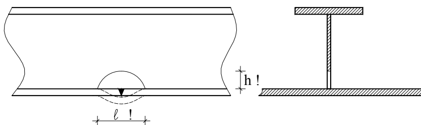
Figure 9.11: Plate buckling at too large cut-out
