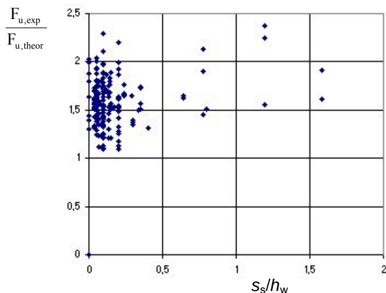
Figure 6.12: Test results over prediction as function of patch length over web depth
