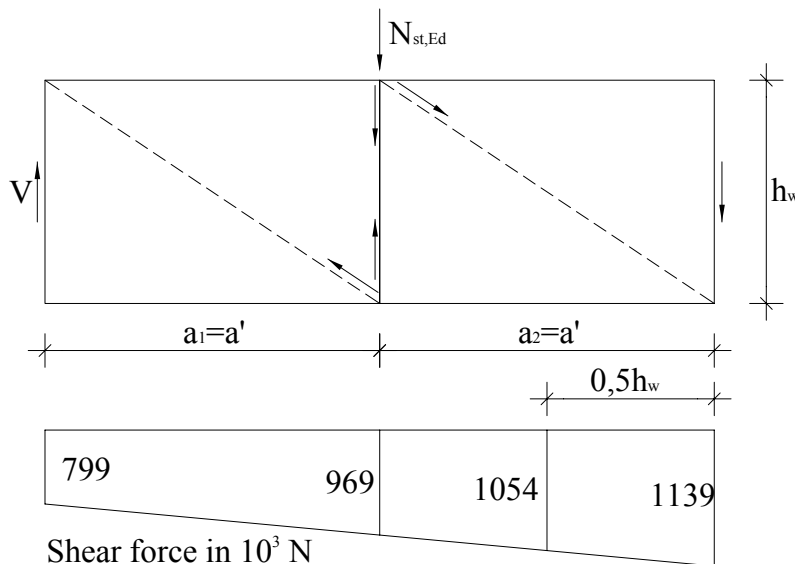
Figure 17.21: Intermediate transverse stiffener – shear force
