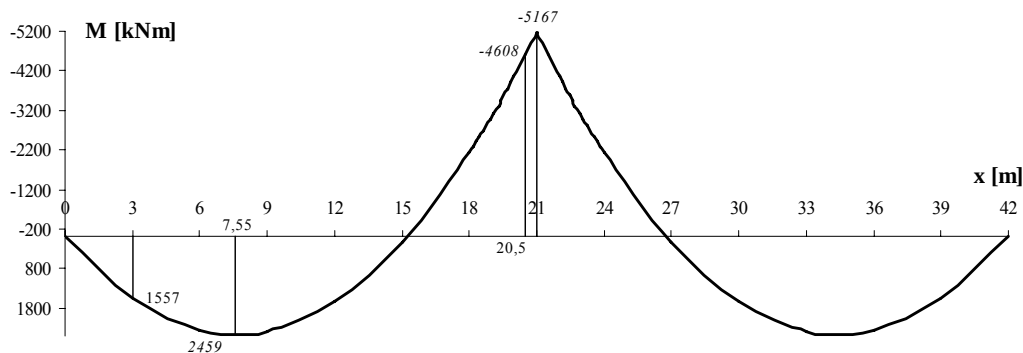
Figure 17.4: Bending moment
