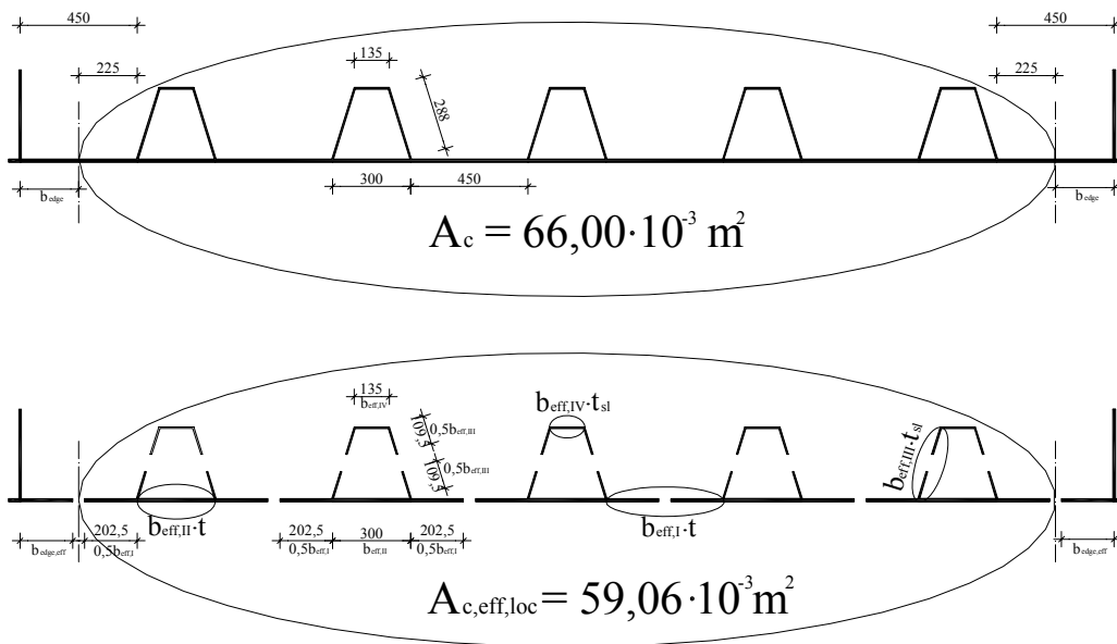
Figure 16.4: Cross section considered and A_{c,\text{eff},\text{loc}}
