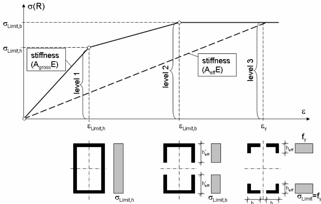
Figure 2.7: Development of effective cross-sections versus the strains \varepsilon
