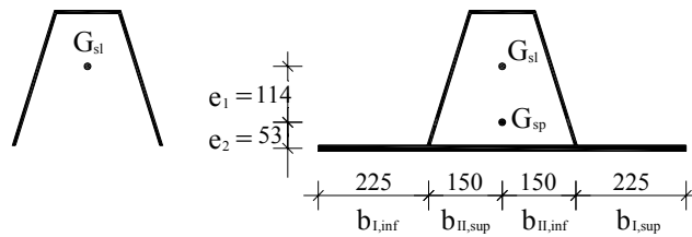
Figure 16.8: Distances e_1 and e_2
