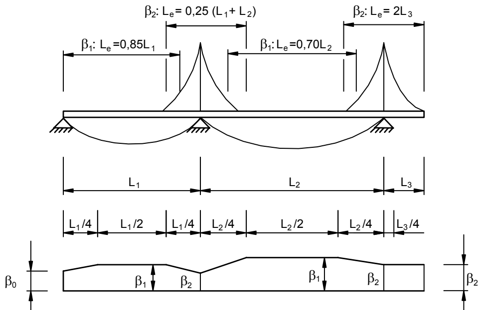
Figure 3.16: Moment envelopes
