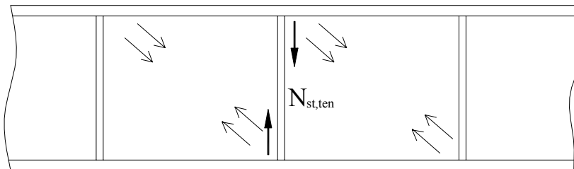
Figure 9.15: Axial force in the intermediate transverse stiffeners
