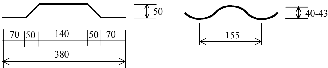
Figure 13.1: Geometry of web plate of Ranabalken, Sweden and Sin-beam, Austria
