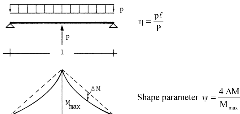
Figure 3.10: Modules representing simply supported beams
