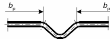
(e) notional flat width b_p of flat parts adjacent to flange stiffener
