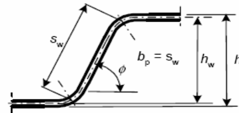
(c) notional flat width b_p for a web ( b_p = \text{slant height } s_w )
