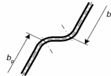
(d) notional flat width b_p of plane parts adjacent to web stiffener
