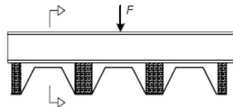
d) Example of method of applying a line load
