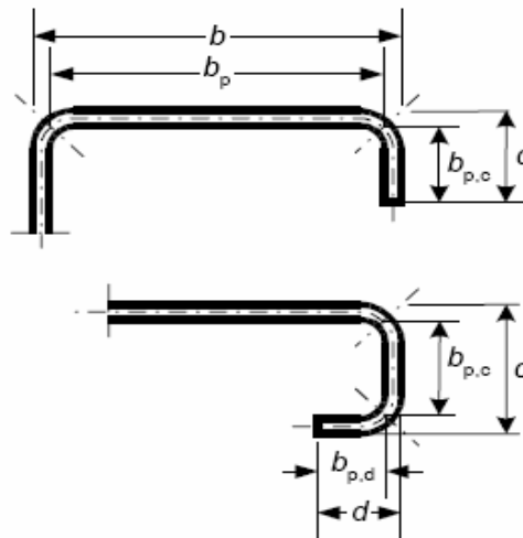
(b) notional flat width b_p of plane parts of flanges
