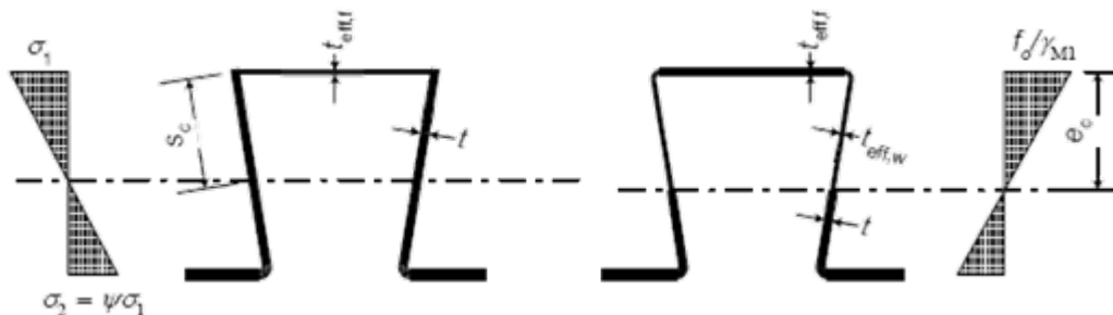
Effective cross-section for resistance to bending moments
